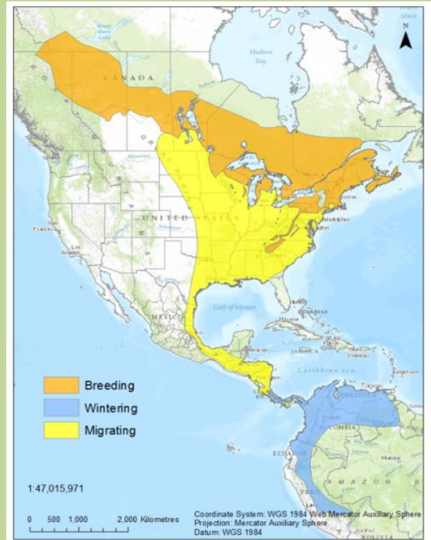
Global range of Canada Warbler showing breeding, migrating, and wintering distribution (adapted from BirdLife International and NatureServe (2013), using data from Haché et al. (2014) and eBird (2014)).
